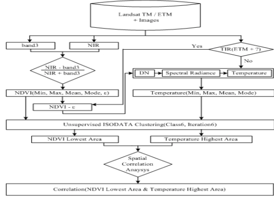
Figure 1. Proposed calibration algorithm for the correlation analysis in multi-bandwidth images
