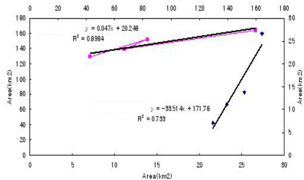
Figure 2. Correlation between the highest LST and the lowest NDVI
